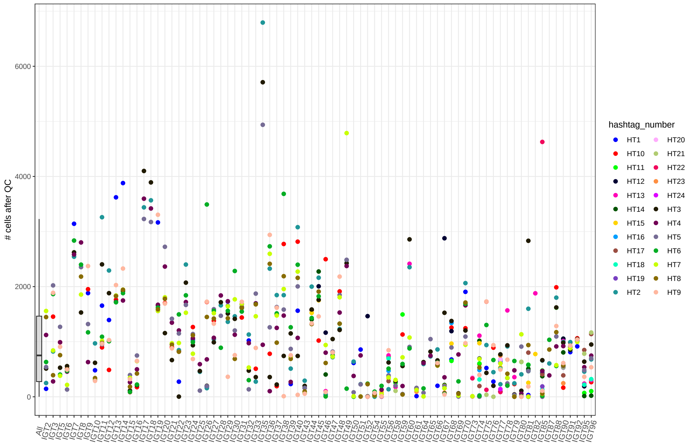
Cells after QC by IGT and sample
